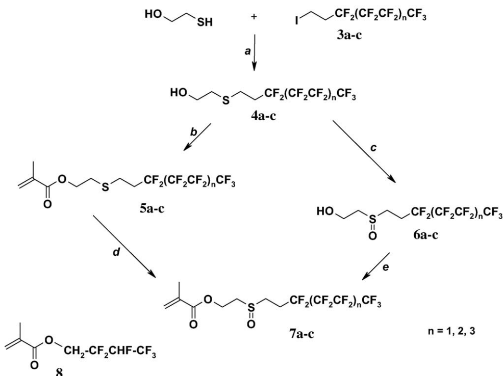
Scheme 1. Preparation of new monomers 7a–c : (a) NaOH, t -BuOH, reflux, 3 h, 86–90%; (b) methacryloyl chloride, \text{Et}_3\text{N} , \text{Et}_2\text{O} , r.t., 5 h, 94–96%; (c) \text{NaIO}_4 , MeOH, water, 0 °C, 1 h, r.t., 5 h, 97–98%; (d) \text{NaIO}_4 , MeOH, water, 0 °C, 1 h, r.t., 5 h, 94–96%; (e) methacryloyl chloride, \text{Et}_3\text{N} , \text{Et}_2\text{O} , r.t., 5 h, 91–94%.
